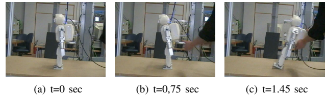
Fig. 11. HOAP3 experiments with in-phase coefficients at high frequency ( f = 1\text{Hz} , BoS = 1\text{cm} , A_t = 5\text{cm} ). The robot cannot maintain its balance and falls backward.
