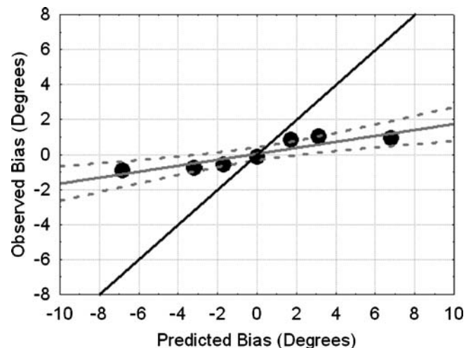
Fig. 2 Mean observed angular constant errors as a function of predicted angular eigenvector deviation ( y=0.17x )
